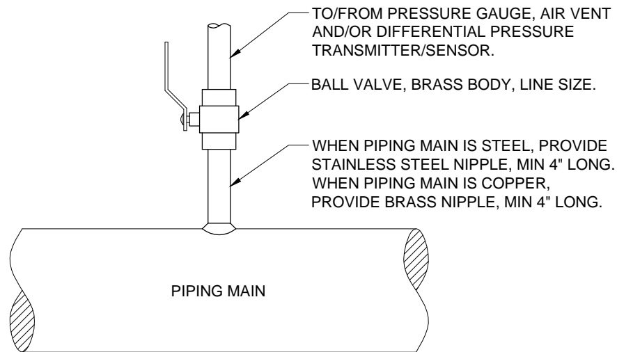
- TYPICAL MAIN PIPE TAPPING DETAIL - SCALE: NONE
