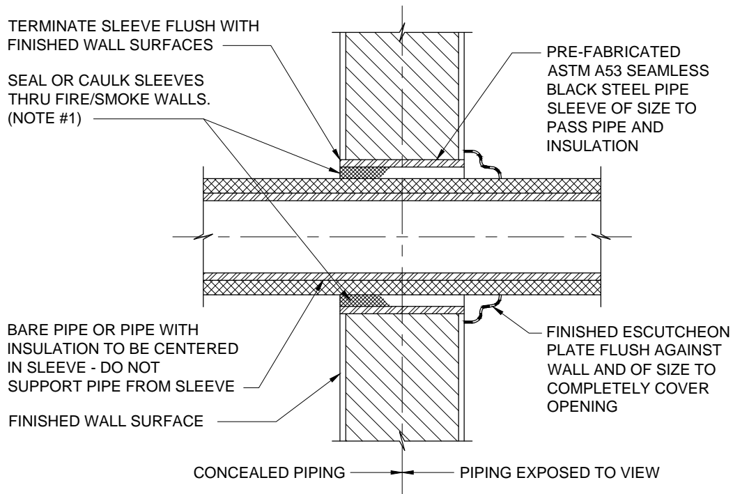
PIPE SLEEVE THRU INTERIOR WALL SCALE: NONE
