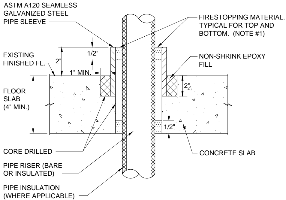
- PIPE SLEEVE THRU FLOOR - SCALE: NONE
