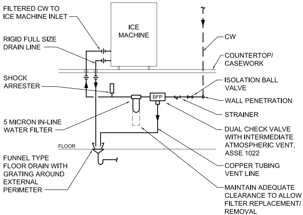
ICE MACHINE PIPING DETAIL SCALE: NONE
