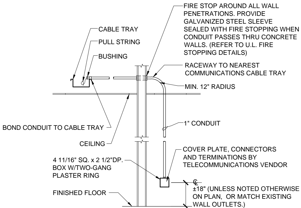
TYPICAL COMMUNICATIONS / DATA OUTLET INSTALLATION DETAIL 0 NOT TO SCALE
