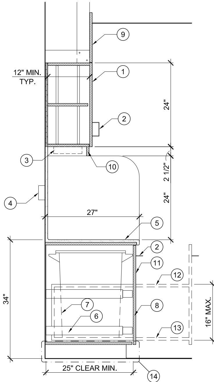
PULL OUT WASTE/LINEN CABINET - SECTION
