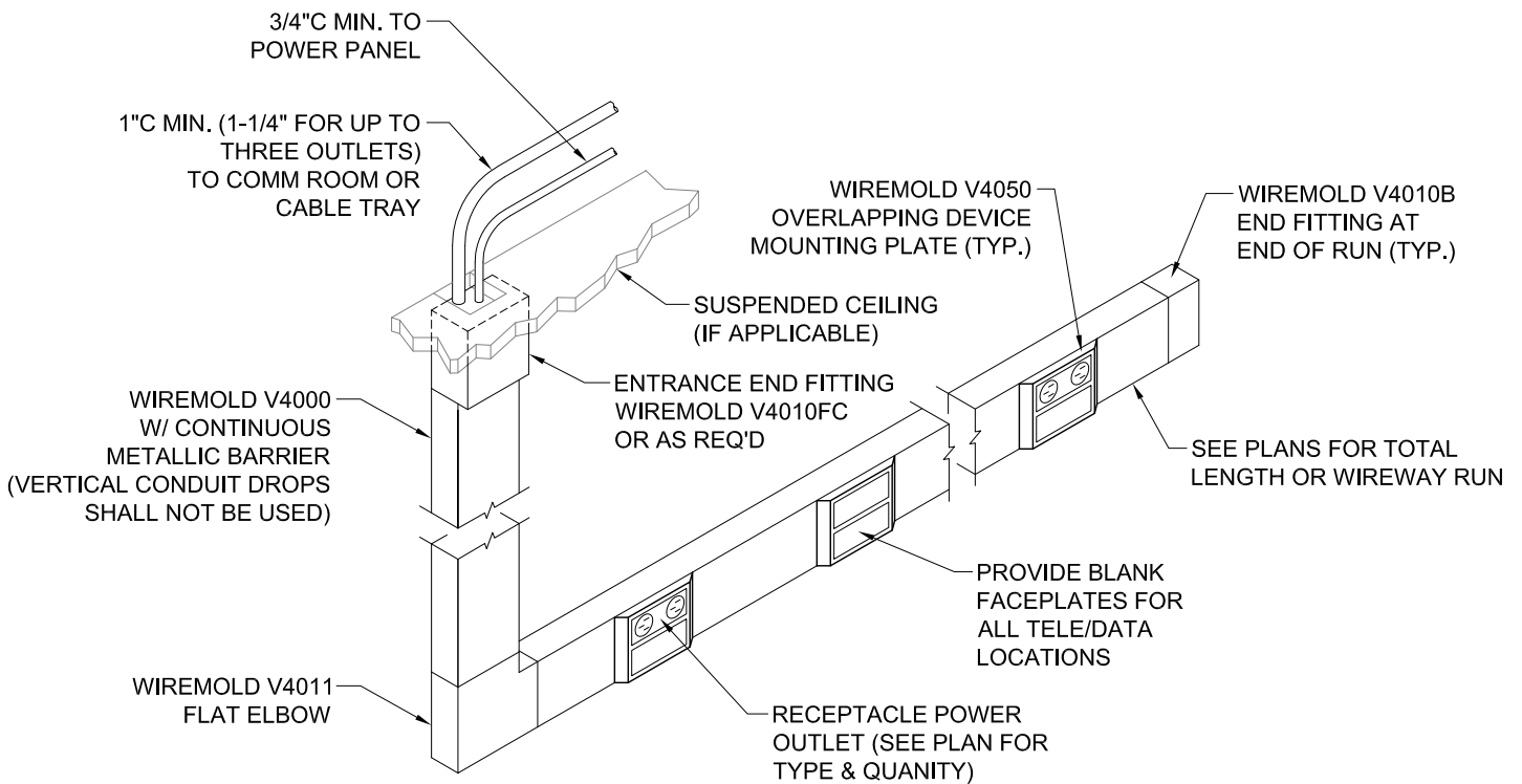
○ - - - TYPICAL DUAL CHANNEL WIREWAY FOR EXISTING WALL 0 NOT TO SCALE
