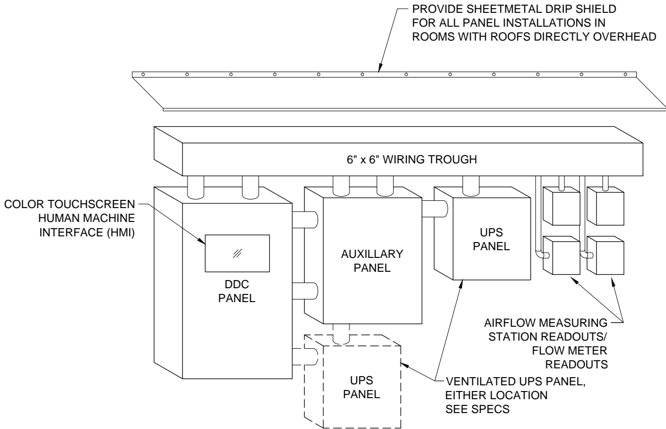
○ - TYPICAL DDC PANEL ASSEMBLY 0 NOT TO SCALE
