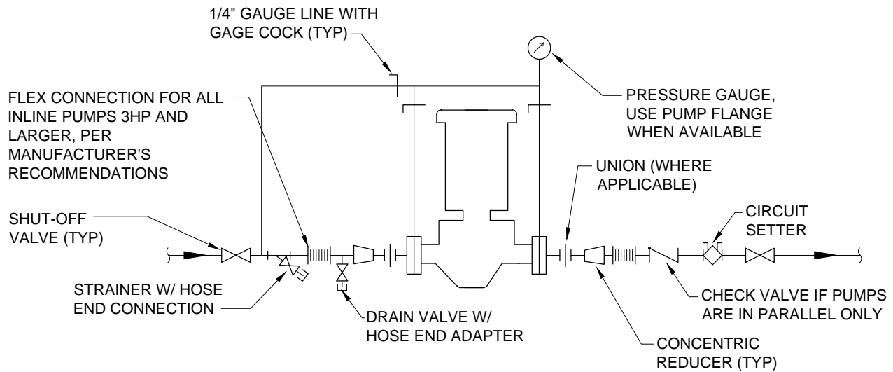
- INLINE PUMP PIPING DIAGRAM - SCALE: NONE
