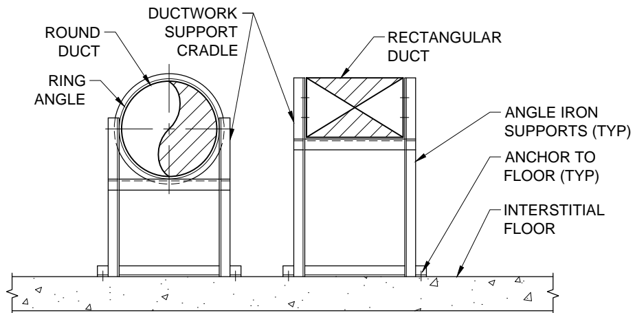
- TYPICAL INTERSTITIAL - LEVEL DUCT SUPPORTS - SCALE: NONE
