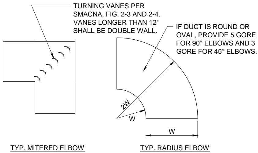
- DUCT ELBOW DETAIL - SCALE: NONE
