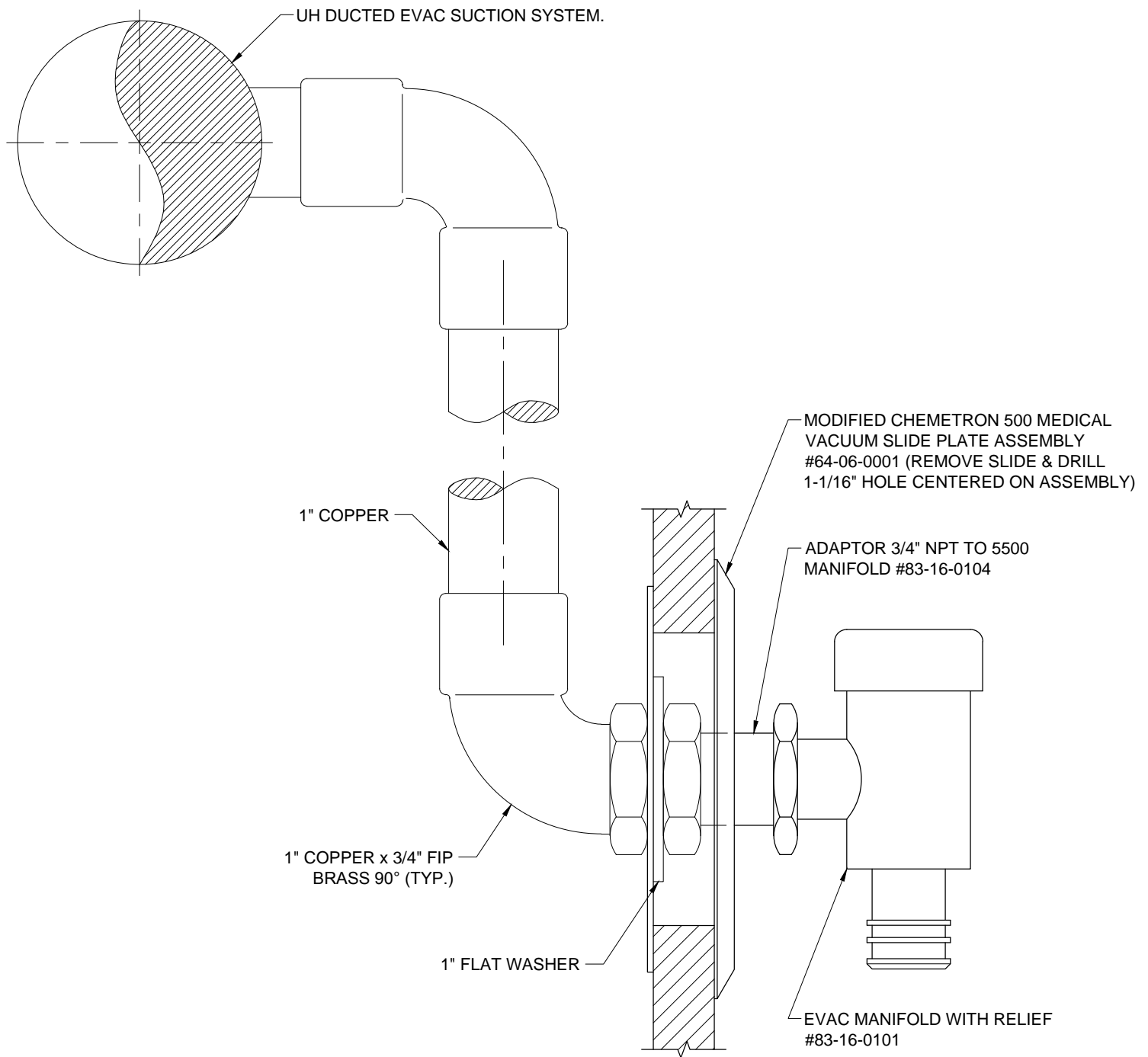
EVAC OUTLET DIAGRAM SCALE: NONE
