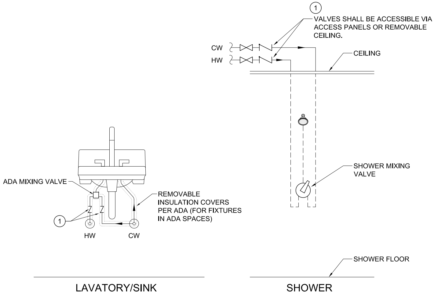
- TYPICAL MIXING VALVE DETAIL - SCALE: NONE
