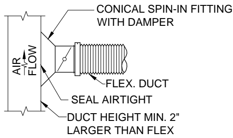
○ TYPICAL DUCT TAP DETAILS 0 NOT TO SCALE
