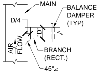
○ TYPICAL DUCT TAP DETAILS 0 NOT TO SCALE
