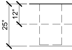
PULL OUT WASTE/LINEN CABINET - PLAN 0 1' 2' 4'
