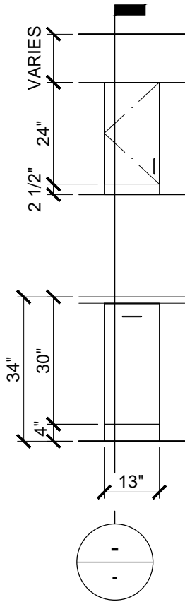
PULL OUT WASTE/LINEN CABINET - ELEVATION 0 1' 2' 4'
